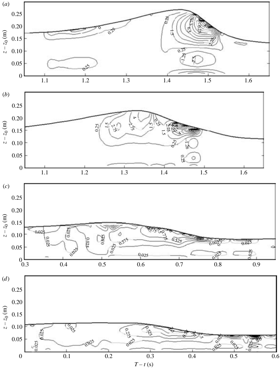
FIGURE 11. Residual turbulent shear stress ( -\rho u'w' ), ( \text{N m}^{-2} ), contour plots for initial breaking at (a) x = 5.54 and (b) 5.737 m and bores at (c) x = 6.796 and (d) 7.200 m.
