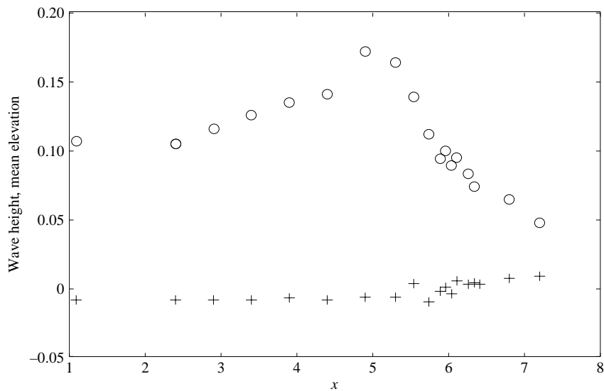
FIGURE 2. Variation of \circ , wave height and + , mean elevation (m), with distance x (m), from the wavemaker.
