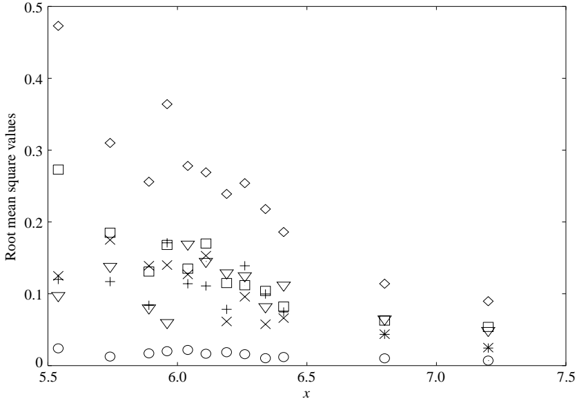
FIGURE 17. Variation of r.m.s. values of terms I (◇), II (+), III (□), IV (×), V (▽) in (9) and overall balance (○), ( \text{m}^2 \text{s}^{-2} ), with distance x (m) from the wavemaker.
