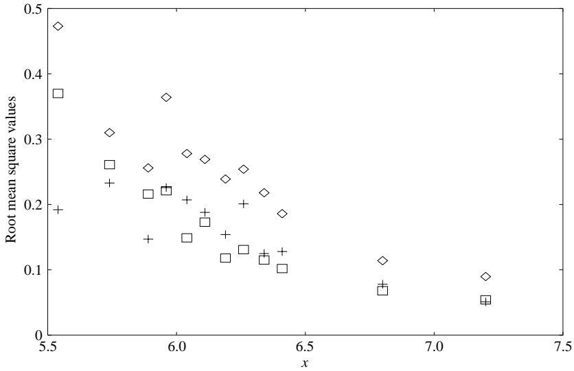
FIGURE 18. Variation of r.m.s. values of terms I (◇), II-V (+), III-IV (□), ( \text{m}^2 \text{s}^{-2} ), with distance x (m) from the wavemaker.
