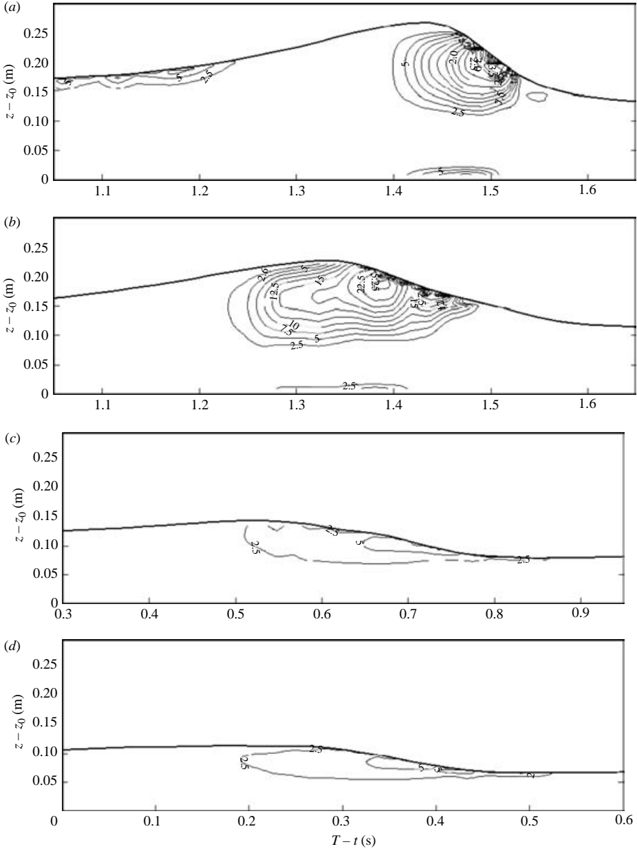
FIGURE 10. Vertical residual turbulent normal stress ( \rho\tilde{w}^2 ), ( \text{N m}^{-2} ), contour plots for initial breaking at (a) x = 5.54 and (b) 5.737 m and bores at (c) x = 6.796 and (d) 7.200 m.
