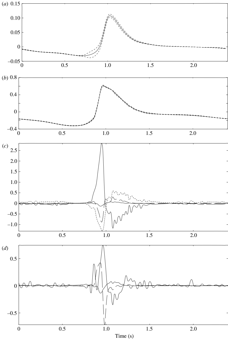
FIGURE 13. Variations of (a) surface elevation, (b) velocity (both with \pm standard deviation \sigma shown as dashed lines) and (c) momentum terms, —, I; ---, II; \dots , III, (d) —, IV; ---, V and overall balance with time for position x = 5.54 m shown as a full line.
