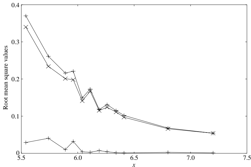
FIGURE 19. Variation of the r.m.s. Lagrangian acceleration term, \int_{z_b}^{\bar{\eta}} D\bar{u}/Dt dz , I + II - V, (×); r.m.s. 'total' pressure gradient term, III-IV, (+); and the r.m.s. of the surface stress term, VI, (lower +), ( \text{m}^2 \text{s}^{-2} ) with distance x (m) from the wavemaker.
